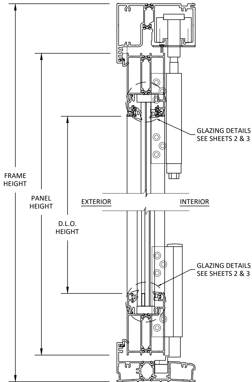
A 8 VERTICAL SECTION STANDARD SILL - NOT RATED FOR WATER INSWING DOOR
