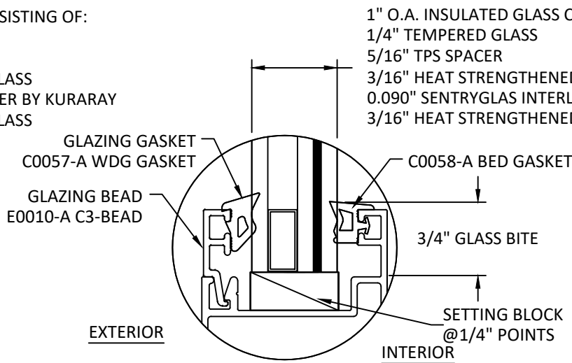
GLAZING DETAIL 9
