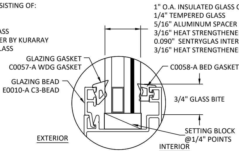
GLAZING DETAIL 8
