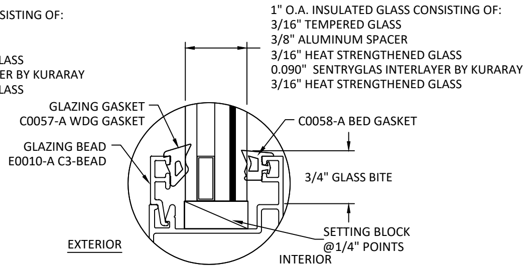
GLAZING DETAIL 4
