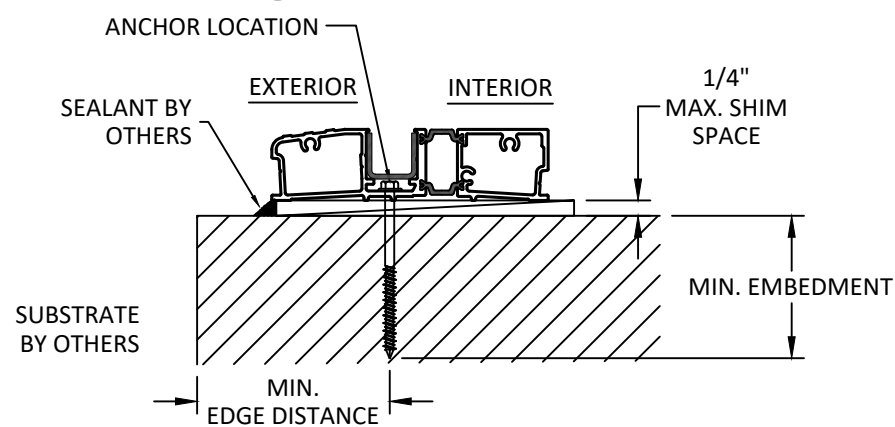
B 11 ANCHOR DETAIL STANDARD SILL - THROUGH FRAME
