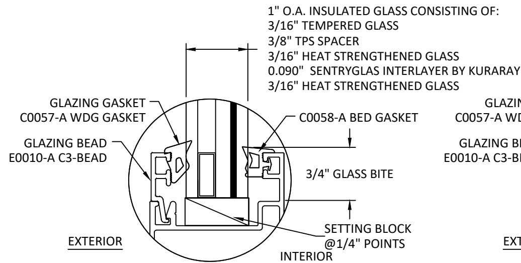
GLAZING DETAIL 3
