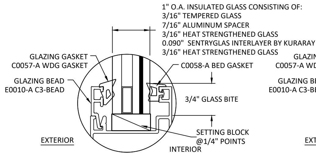
GLAZING DETAIL 5
