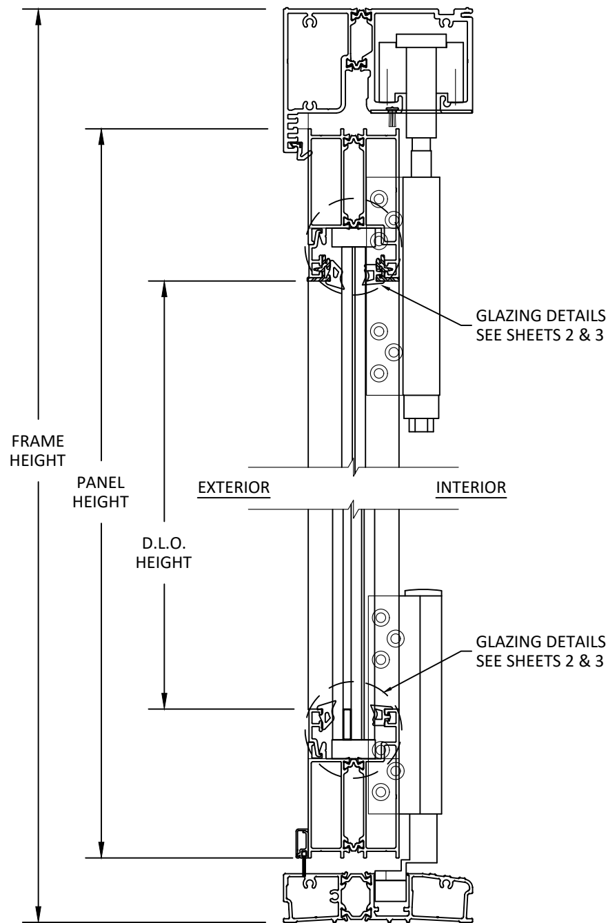
B 8 VERTICAL SECTION MODIFIED STANDARD SILL - NOT RATED FOR WATER INSWING DOOR
