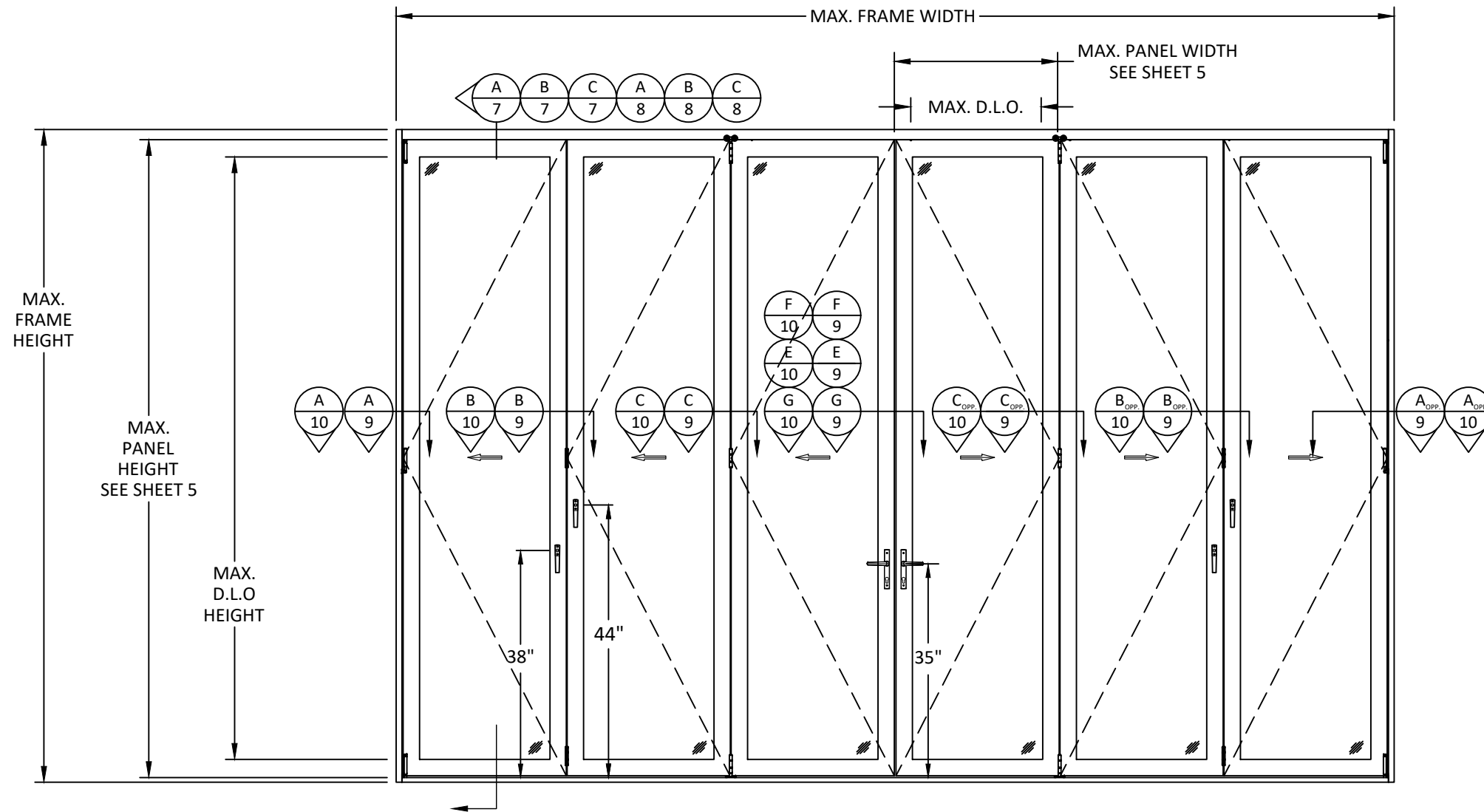
ELEVATION INSWING/OUTSWING UNIT 1
