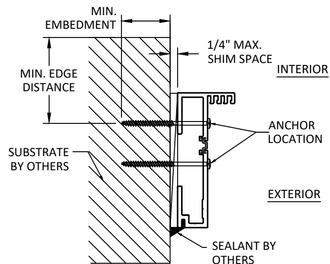
C 11 ANCHOR DETAIL JAMBS - THROUGH FRAME
